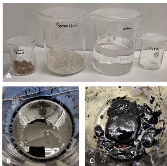
Figure 1. A) Hydrothermal liquefaction reactants, showing ground spruce bark, ground spruce wood, water, and catalyst. B) Bio-oil from continuous HTL under supercritical conditions (400C, 300 bar). C) Bio-oil from continuous HTL under sub-critical conditions (350C, 300 bar).
