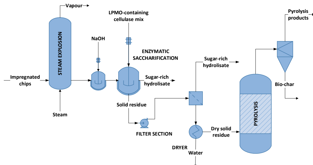
Figure 4 - Simplified layout of the investigated upstream processes of a softwood-based biorefinery. The picture does not include the impregnation step prior to the steam explosion.
