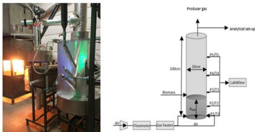
Figure: 20 kW bubbling fluidized bed gasification (BFBG)
