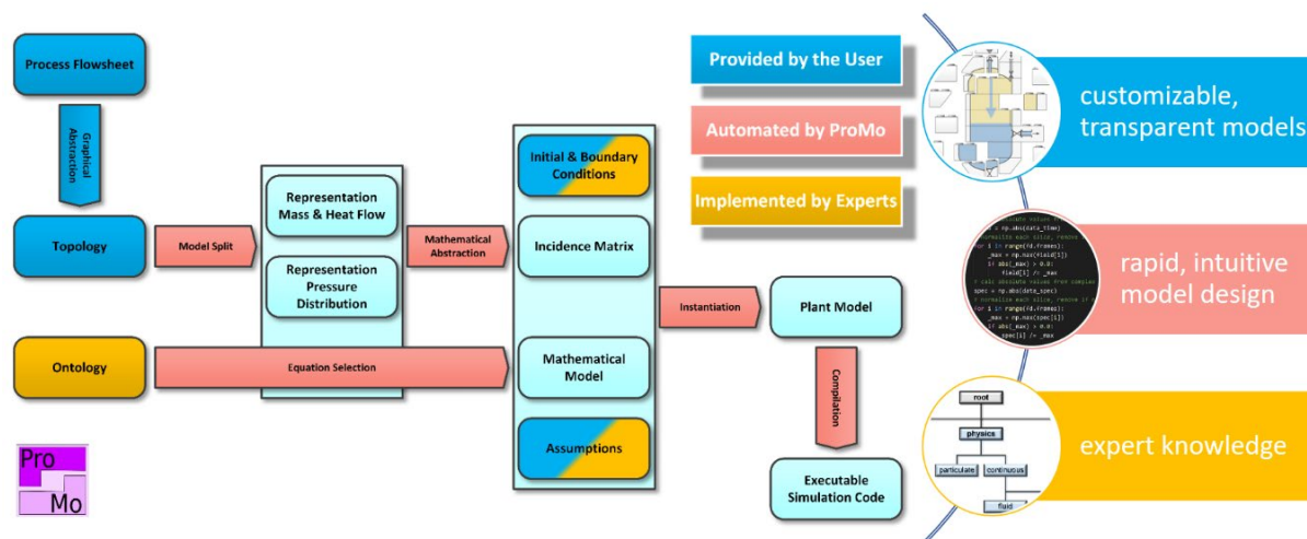
Figure 3: The composition of the modelling suite ProMo
