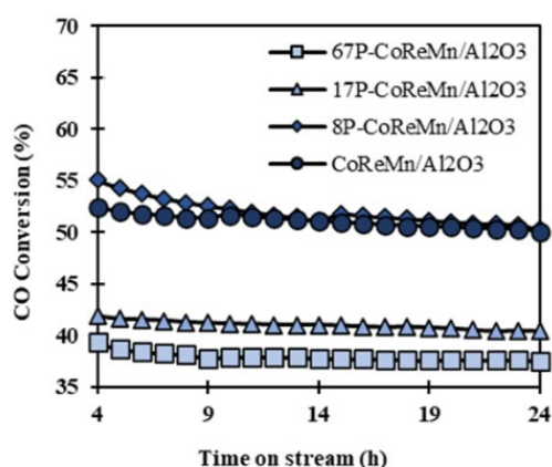
Figure: CO conversion in the FTS over a CoMn/alumina catalyst with different loadings of phosphorus.
