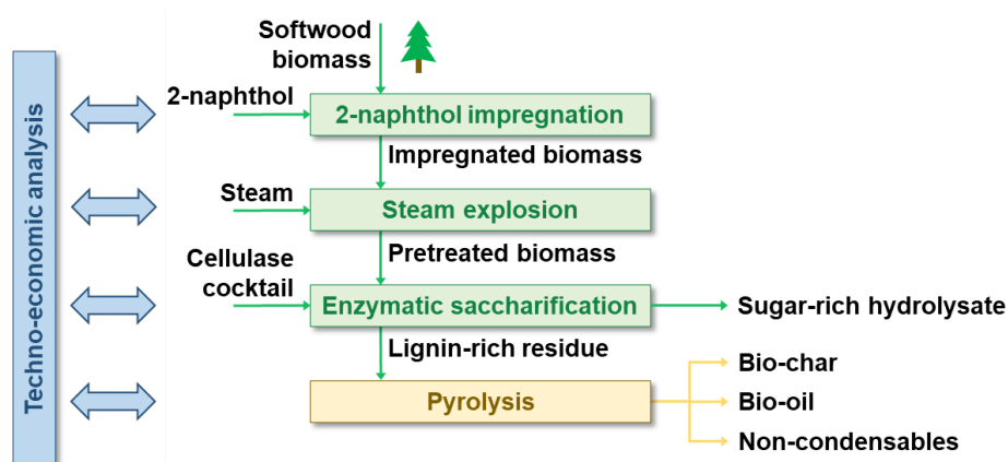
Figure 3.2.1: The process scheme of the combined biochemical and thermochemical conversion route. Softwood impregnation with the carbocation scavenger 2-naphthol prior to steam explosion enabled complete saccharification of the pretreated feedstock, partly due to improved LPMO activity, and yielded high-quality saccharification rests for valorization by pyrolysis.
