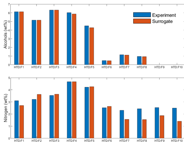
Figure 7: Comparison of the surrogate formulation and the fuel sample (experiment). Top: alcohol content, bottom: nitrogen content.
