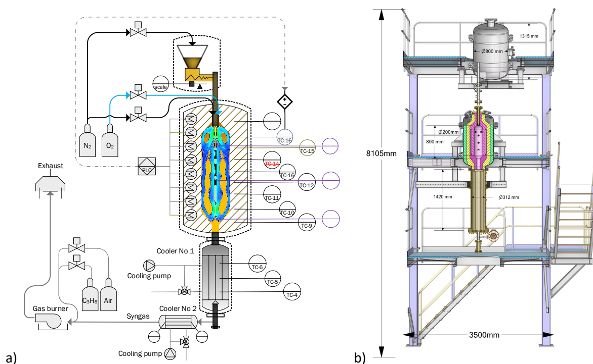
Figure 2: a) The ER reactor and its subsystems b) The EFR is built into a frame for easy access to the hopper and for reactor for cleaning and maintenance.
