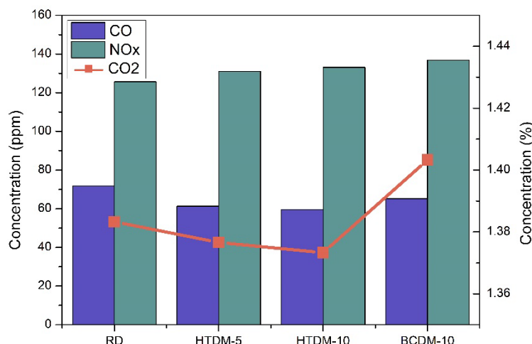
Figure 5: Emission measurements of reference Diesel (RD) and the HTL/RD fuel blends.
