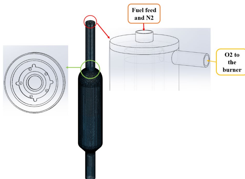
Figure: Boundaries for the inlet of the EF reactor designed in a CPFD model
