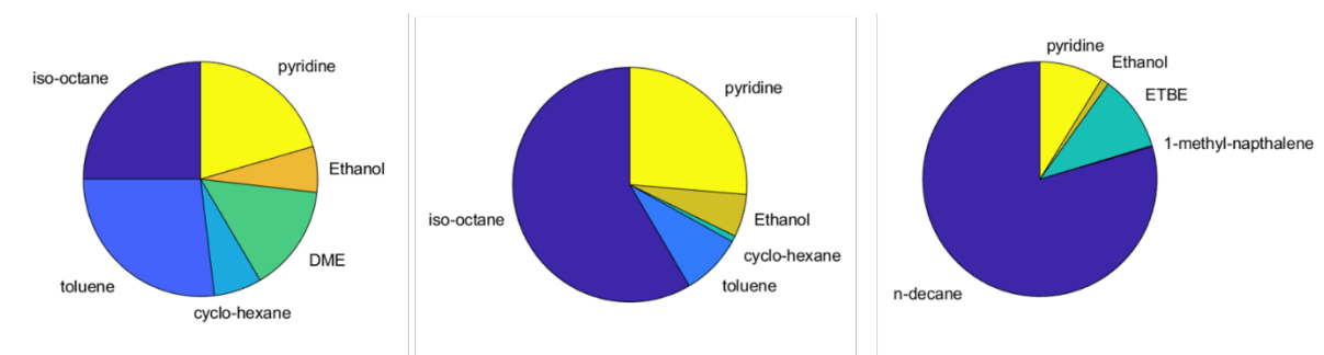
Figure 6: Exemplary surrogate composition from left to right: gasoline, aviation fuel, diesel fuel.
