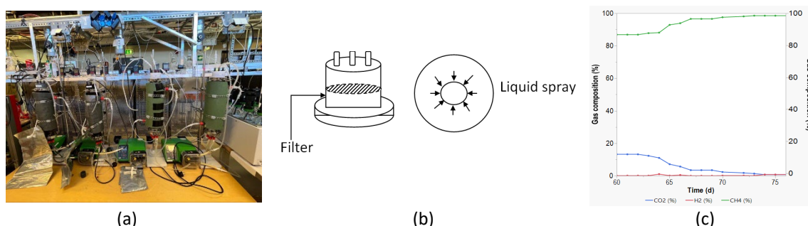
Figure 3.4.1: Modified trickle bed reactors for biogas upgrading. (a) The experimental setup; (b) the 3D-printed reactor head with a filter incorporated; (c) example output of the online gas composition measurement.
