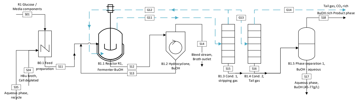
Figure 5.2.2: Butanol reactor
