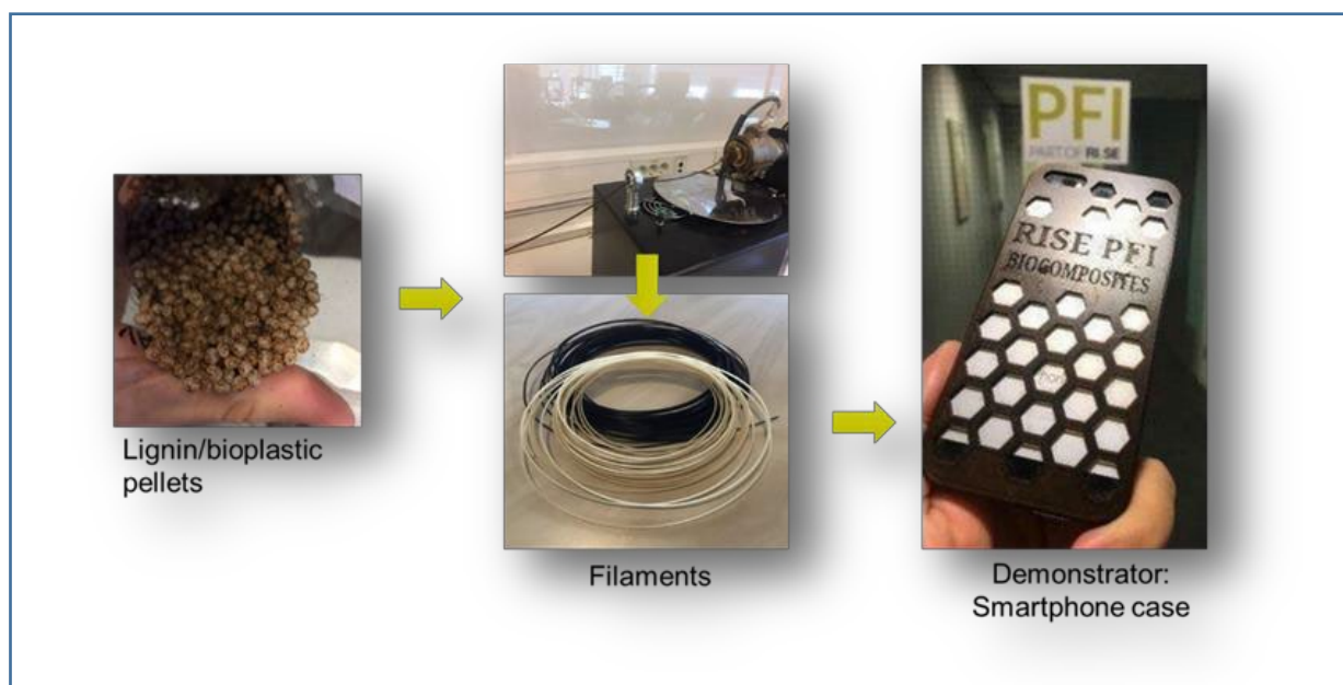
Figure 3.1.1: Left) PLA/lignin pellets. Middle) Extrusion of PLA/lignin filament. Right) 3D printed demonstrator of PLA/lignin biocomposites.
