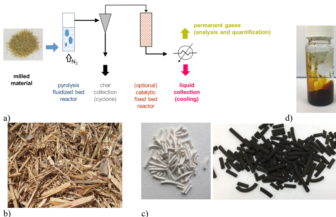
Photo: The Bio4Fuel research team at RISE PFI are exploring catalytic pyrolysis of waste wood for producing a biocrude quality suitable for upgrading in to a marine or aviation drop in fuel. a) Principal diagram for the continuous bench scale fast pyrolysis reactor system. b) Waste wood feedstock. c) Fresh and used zeolite catalyst pellets with coke. d) Low-viscous biocrude sample produced from waste wood.
