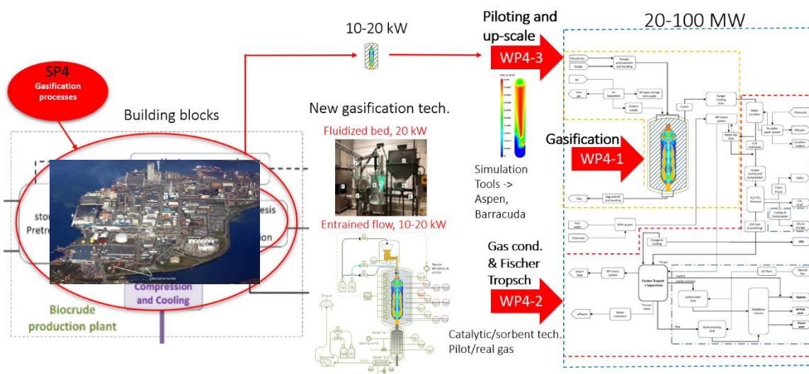
Figure: The main outcome of the work in SP4 is the specification of a full-scale industry cluster, integrated process solution, based on thermochemical conversion of selected carbonaceous feedstocks (by gasification, producing high-value clean syngas to supplement existing sidestreams...or converted to a liquid fuel through Fischer Tropsch).
